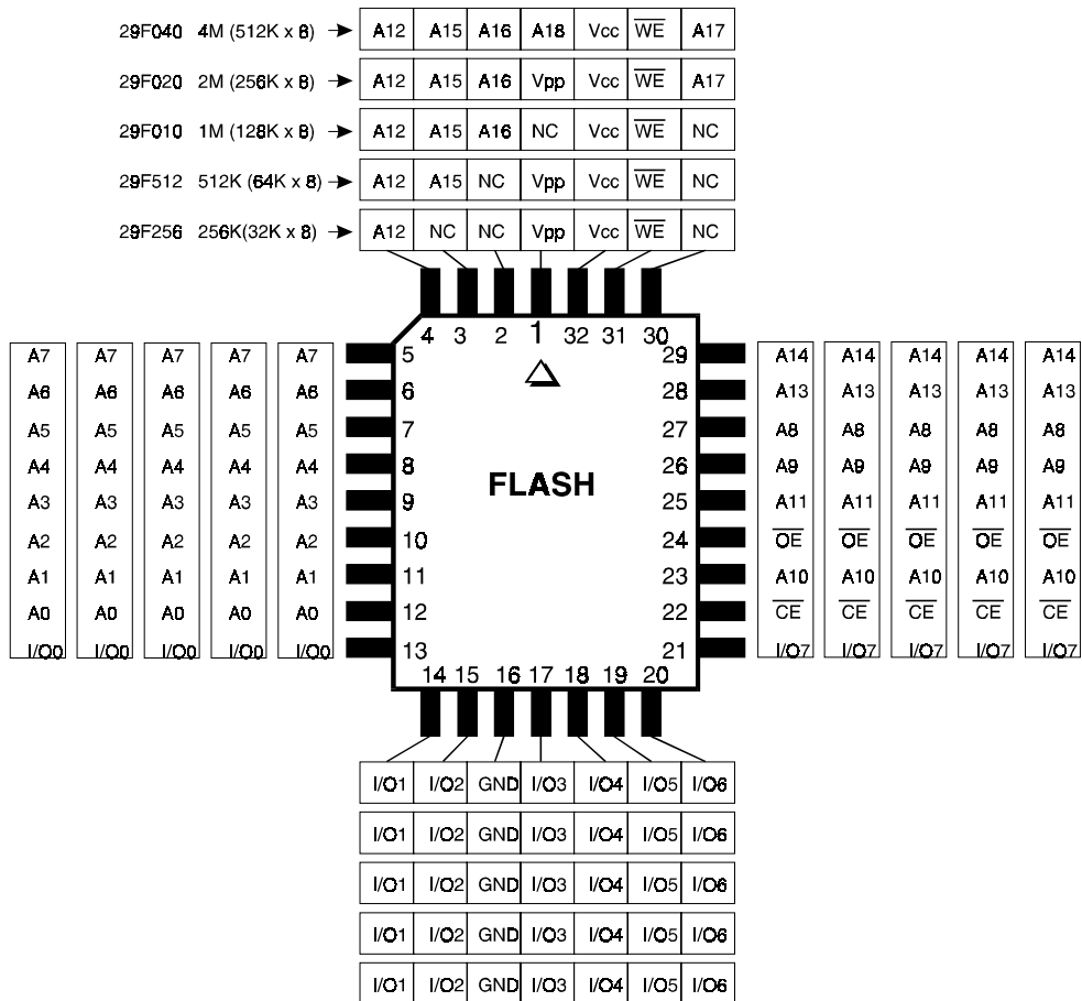
Standard PLCC FLASH pinouts (29F256-29F040)
