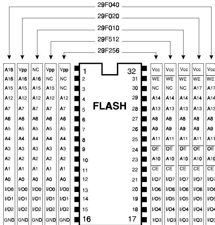
Standard FLASH Pinouts (29F256 - 29F040)
