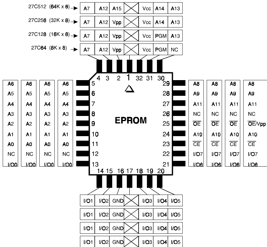
Standard PLCC EPROM pinouts (27C64-27C512)
